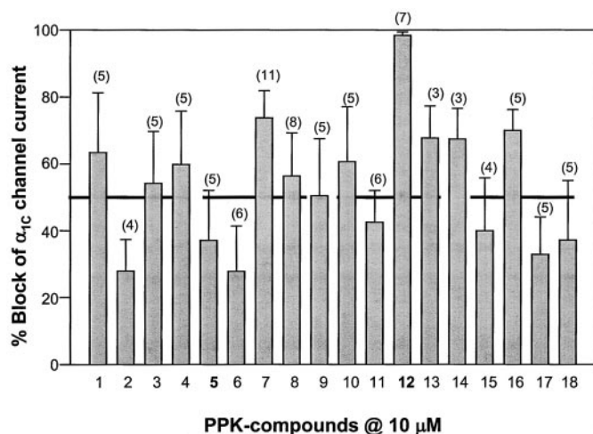
Fig. 2. Inhibitory effects of the PPK series on L-type ( \alpha_{1C} + \alpha_{2-\delta} + \beta_{1b} ) calcium channels transiently expressed in tSA-201 cells. Whole-cell currents were recorded in 5 mM external barium by stepping from a holding potential of -80 mV to a test depolarization of 0 mV. The degree of block was determined from the percentage of peak current inhibition obtained in the presence of each of the compounds. The bars reflect means, error bars are S.D., and numbers in parentheses indicate the number of experiments.
