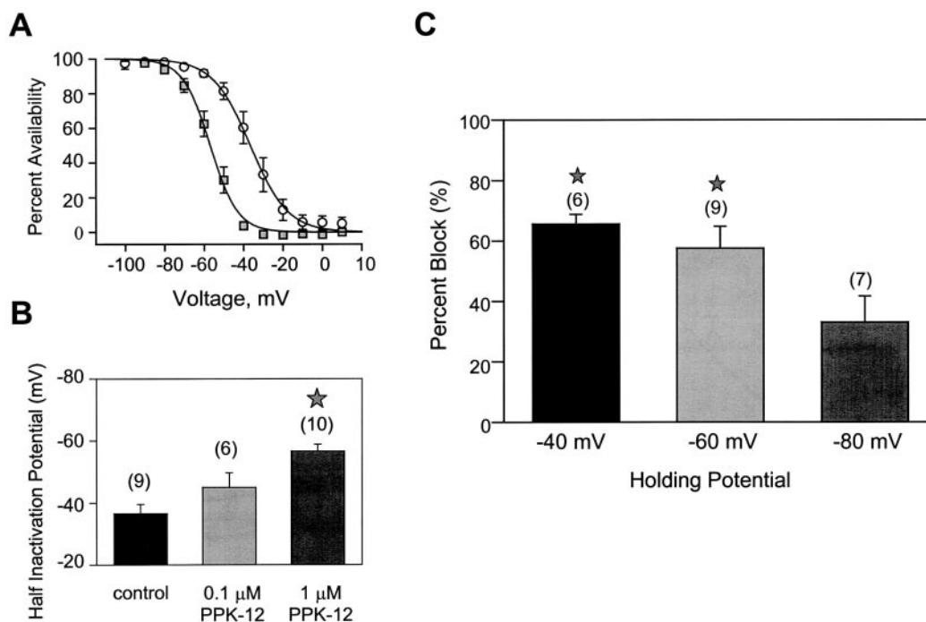
Fig. 4. Dependence of PPK-12 block of L-type calcium channel on holding potential. A, ensemble steady-state inactivation curves obtained in the absence (○) and presence (□) of 1 \mu M PPK-12. The data were fitted with the Boltzmann equation (solid lines). The half inactivation potentials obtained from the fits were -36.5 mV and -56.8 mV in the absence and the presence of 1 \mu M PPK-12, respectively. In each case, steady-state inactivation curves in the absence and presence of PPK-12 were recorded from the same cell for a total of 10 cells. Error bars are S.E. B, dependence of half-inactivation potential on the concentration of PPK-12. The asterisks indicate statistical significance relative to control ( P < 0.05 ; Student's t test). C, dependence of the blocking effects of 300 nM PPK-12 on the holding potential. Note the significant increase in the degree of block ( P < 0.05 ) at more depolarized membrane potentials. The asterisks indicate significance relative to the data obtained at -80 mV ( p < 0.05 ).
