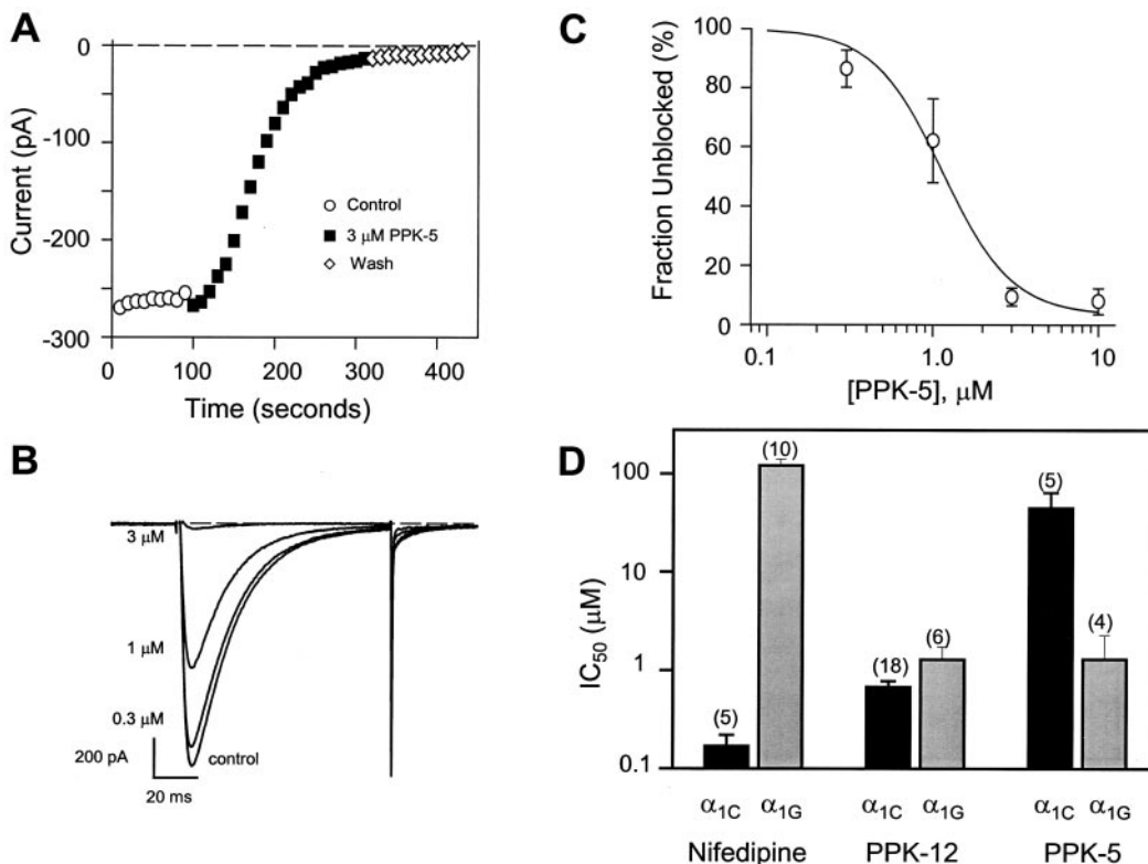
Fig. 6. Block and selectivity of PPK-5 for T-type calcium channels. A, representative time course of block of T-type calcium channel by 3 \mu\text{M} PPK-5. Note the lack of reversibility. B, current records obtained in the absence and presence of PPK-5 under the same conditions as those in Fig. 5B. C, dose dependence of PPK-5 action on transiently expressed T-type channels obtained from 11 different cells. The experimental conditions were the same as in Fig. 5C, the \text{IC}_{50} and Hill coefficient obtained from the fit were 1.14 \mu\text{M} and 2.06, respectively. D, relative selectivities of nifedipine, PPK-12, and PPK-5 among L- and T-type calcium channels. Note that the \text{IC}_{50} values shown on the ordinate are on a logarithmic scale. Error bars are S.E., numbers in parentheses reflect the number of cells used to calculate the means.
