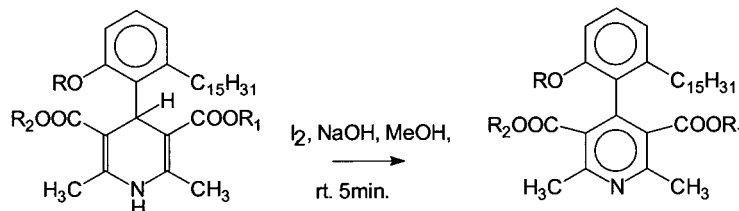
Fig. 1. Synthesis of the series of dialkyl 1,4-dihydro-4-(2'-alkoxy-6'-pentadecylphenyl)-2,6-dimethyl-3,5 pyridine dicarboxylates from anacardic acid as described in detail under Materials and Methods section. In scheme 1, the reagents used in each step were as follows: (\text{CH}_3)_2\text{SO}_4/\text{K}_2\text{CO}_3 , acetone, reflux 3 h (a); \text{LiAlH}_4 , Tetrahydrofuran, reflux 3 h (b); PCC, dichloromethane, rt. 3 h (c); \text{CH}_3\text{COCH}_2\text{COOR}_1/\text{piperidine}/\text{acetic acid} , n -butanol, rt. 3 h (d); and (\text{CH}_3)_2\text{N}(\text{NH}_2)\text{C}=\text{CH}(\text{COOR}_2) , n -butanol, reflux 30 h (e).
