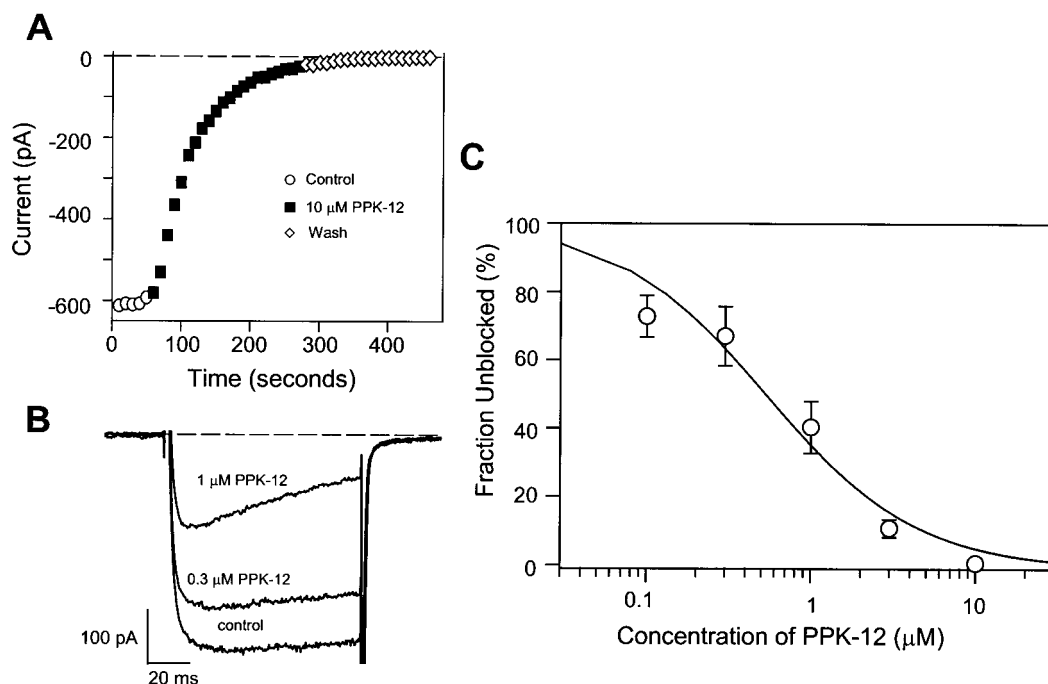
Fig. 2. Inhibitory effects of the PPK series on L-type ( \alpha_{1C} + \alpha_{2-\delta} + \beta_{1b} ) calcium channels transiently expressed in tSA-201 cells. Whole-cell currents were recorded in 5 mM external barium by stepping from a holding potential of -80 mV to a test depolarization of 0 mV. The degree of block was determined from the percentage of peak current inhibition obtained in the presence of each of the compounds. The bars reflect means, error bars are S.D., and numbers in parentheses indicate the number of experiments.
