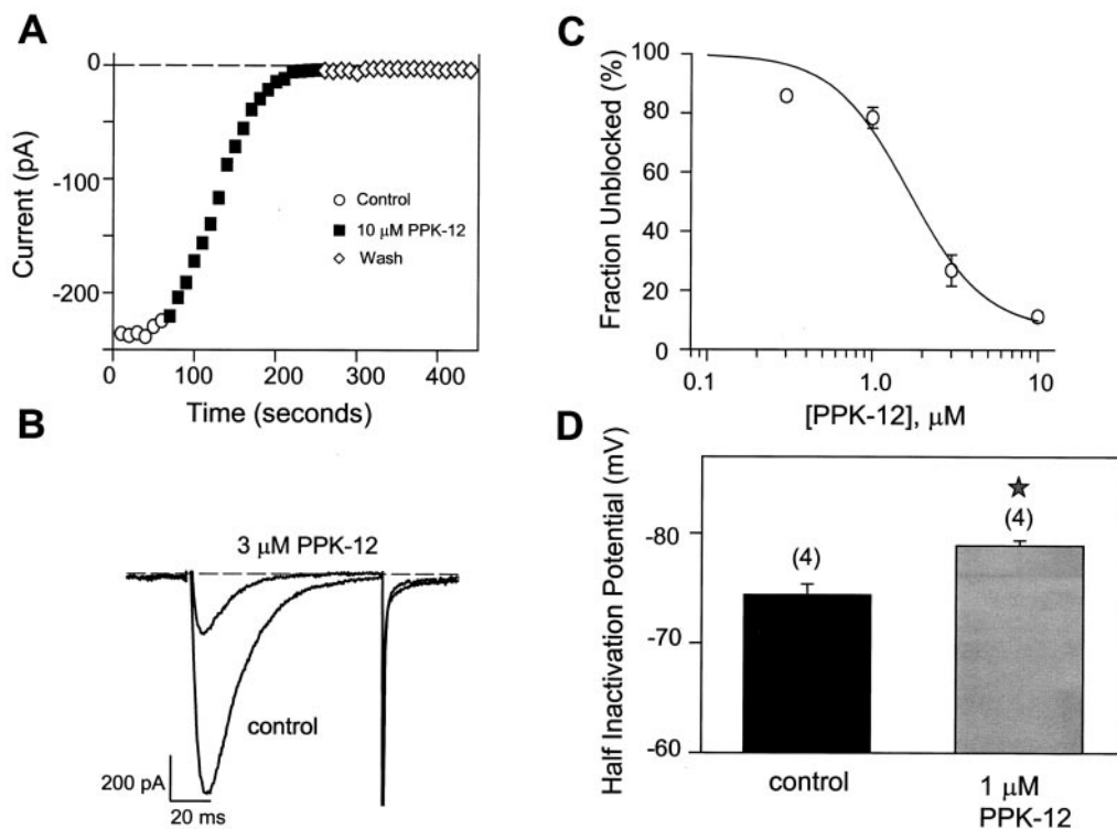
Fig. 5. Effects of PPK-12 on transiently expressed T-type calcium channels. A , representative time course of peak current block induced by 10 \mu\text{M} PPK-12. Note that the inhibition is virtually complete and not reversible after washout. B , effect of 3 \mu\text{M} PPK-12 on whole-cell current records elicited by stepping from -80 mV to a test potential of -20 mV. C , dose dependence of the effects of PPK-12 on transiently expressed T-type calcium channels. Data from 12 experiments are included in the figure. Symbols reflect means from 8 to 12 individual determinations, the solid line is a fit according to the Hill equation ( \text{IC}_{50} = 1.65 \mu\text{M} , n_H = 1.88 ), error bars reflect S.E. D , comparison of the half-inactivation potentials obtained in the absence and presence of 1 \mu\text{M} PPK-12. The asterisk indicates statistical significance ( P < 0.005 , paired Student's t test).
